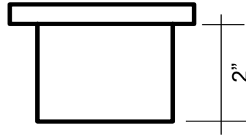
FORM HOLDER - THREE SECTION # FH5317 HORIZONTAL USAGE DEPTH : 2"
