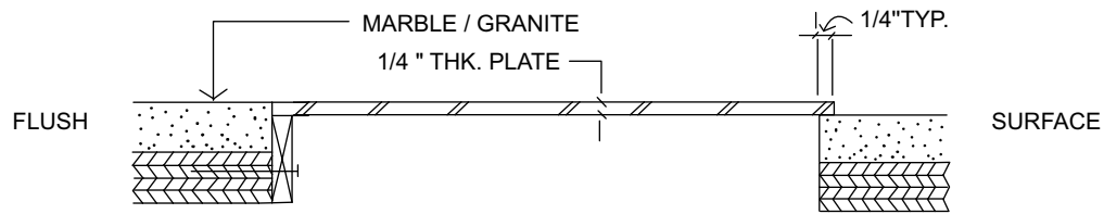
COUNTER CUTOUT FOR MARBLE / GRANITE
